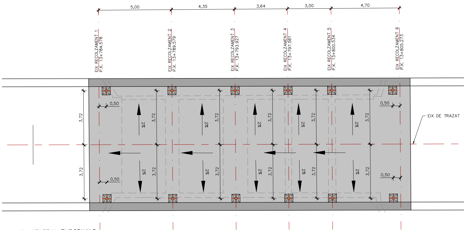
PLANTA GENERAL EMBORNALS
