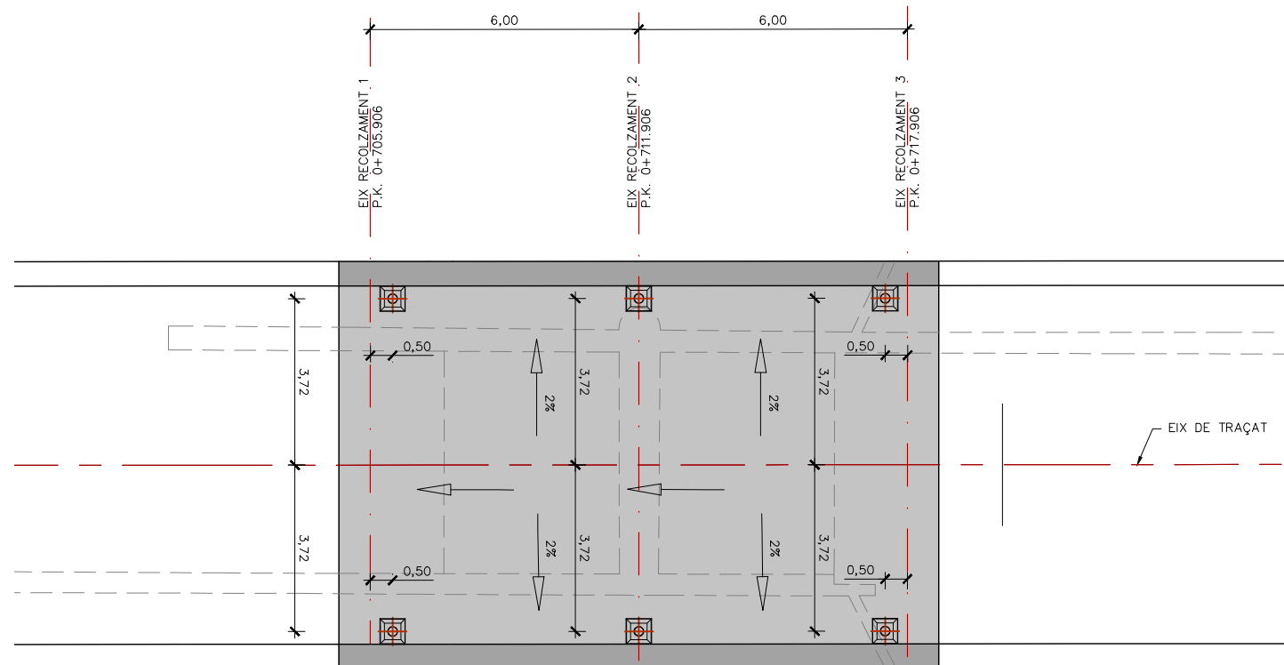
PLANTA GENERA EMBORNALS
